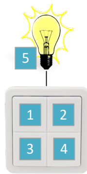
Figure 3. MATRIX endpoints
